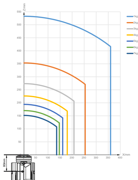
运动空间及外形安装尺寸图 Motion range and installation dimension drawing
