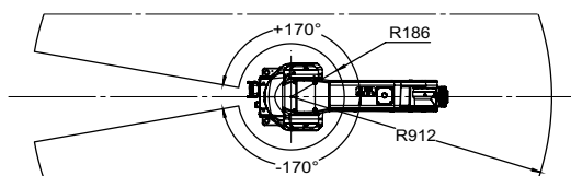
运动空间及外形安装尺寸图 Motion range and installation dimension drawing
