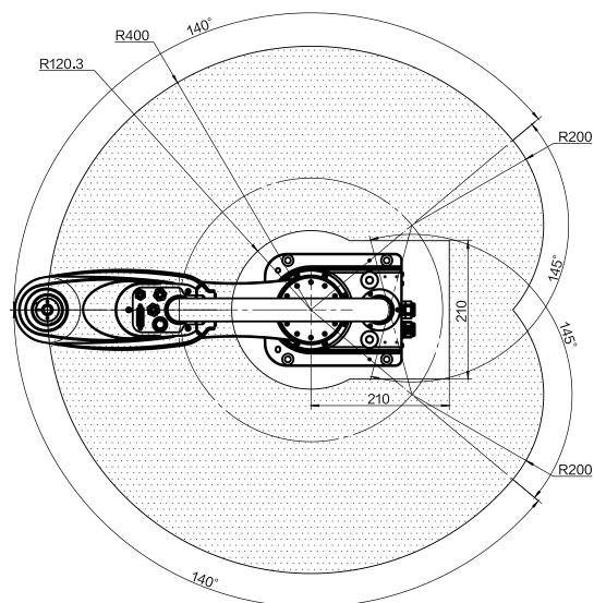
运动空间及外形安装尺寸图 Motion range and installation dimension drawing
